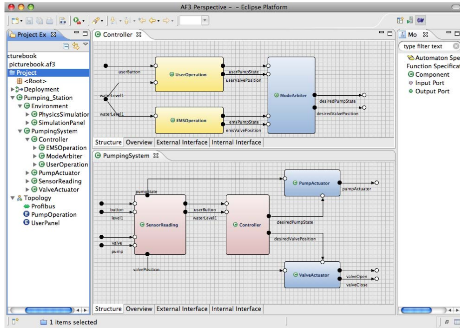
Fig. 3. AUTOFOCUS 3 design tool
