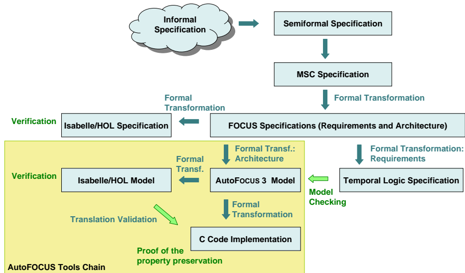
Fig. 1. Development Methodology
